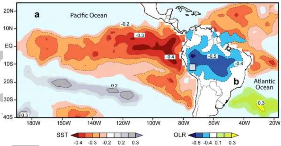
Figure 5. Spatial correlation field between annual (November-October) tree-ring precipitation reconstruction with (a) 2.5 \times 2.5^\circ gridded averaged November-October sea surface temperature (SST) over the equatorial Pacific and tropical Atlantic Oceans for the 1950-2010 period and (b) outgoing longwave radiation (OLR) over South America during the 1979-2010 period. Significant correlations ( p < 0.05 ) are outlined for negative (dashed lines) and positive (solid lines) values. The reconstructed precipitation region is indicated by the square over Peru.
