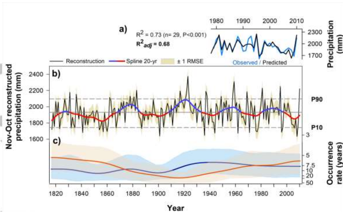
Figure 2. Tree-ring based reconstruction. (a) Comparison between GPCP (blue) and tree-ring reconstructed (black) rainfall for the 1979-2010 period. The coefficient of determination ( R^2 ) and adjusted by degrees of freedom ( R^2_{adj} ) show significant positive correlations between the GPCP precipitation and tree-ring precipitation reconstruction. (b) Reconstruction of the yearly (November-October) precipitation variations in the Amazonian Andes of Peru. This nested tree-ring based reconstruction covers the 1817-2010 period. Mean (1930.9 mm, solid grey line), 90th (2096.8 mm) and 10th (1742.5 mm) percentiles (P90 and P10, dashed lines) are shown for reference in the reconstruction. The shaded area stands for the \pm one root-mean-square error (RMSE), which estimates the uncertainty of the reconstructed series. A 20-year smoothing spline was used to emphasize the low frequency above (blue) and below (red) the mean. (c) Occurrence rate (in years) of severe dry (red) and wet (blue) events for the precipitation reconstruction over the Amazonian Andes of Peru for the last two centuries, calculated for the 10th and 90th percentile thresholds respectively. Shaded areas represent 95% confidence intervals.
